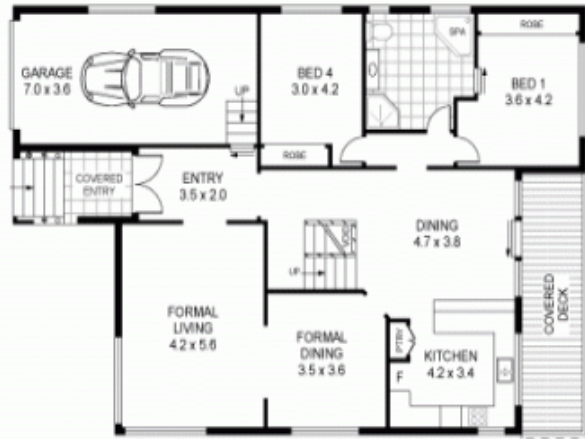
ENTRY LEVEL
