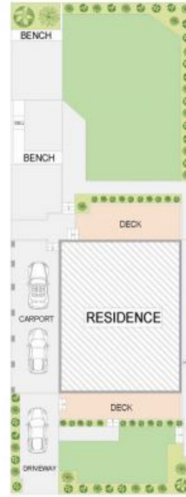
SITE PLAN
