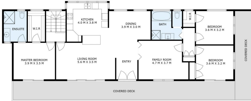
Ground Floor
